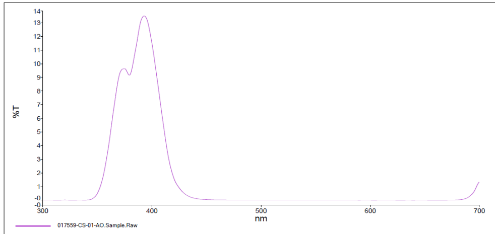
Fig.2.1-1 “2401008926-1” UV-vis spectrogram
